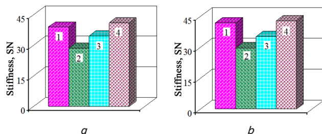
Fig. 2. A dependence of the stiffness of the semi-finished leather on the temperature of its enzymatic plasticizing, °C: 1 – 37; 2 – 54; 3 – 58; 4 – without processing with an enzyme; a – cattle hides; b – LPH
