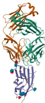
Figure 1.1 – CD47 Structure Diagram
